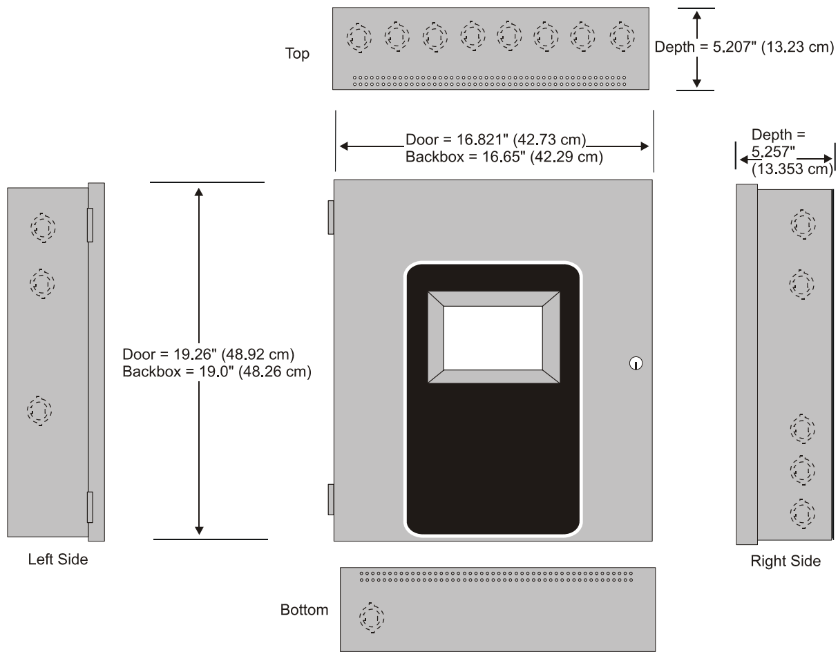
Cabinet Measurements
