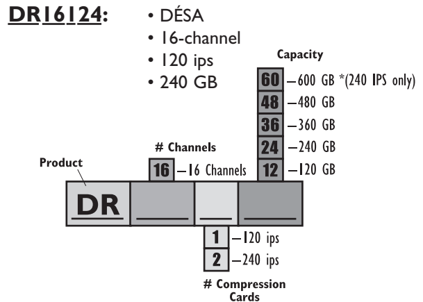
DÉSA Part Numbering Structure
